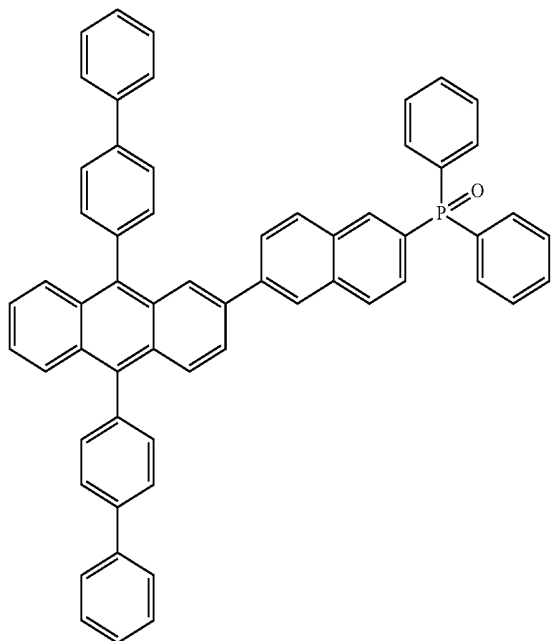
[Formula 1-11]
