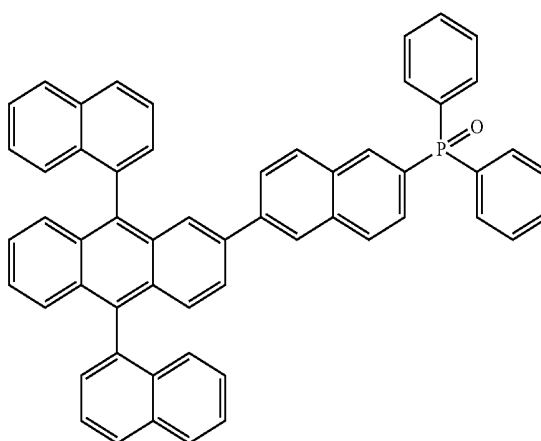
[Formula 1-14]
