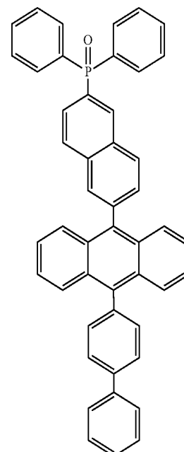
Structural Formula 1-9
