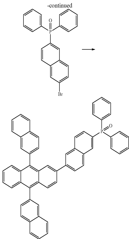
Structural Formula 1-10
