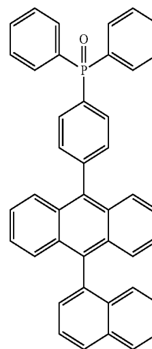
Structural Formula 1-2
