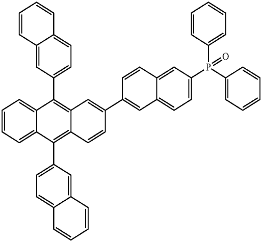
[Formula 1-10]
