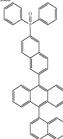
Structural Formula 1-7
