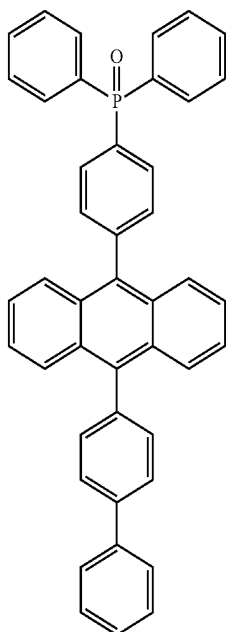
Structural Formula 1-5
