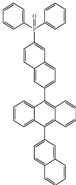
Structural Formula 1-8
